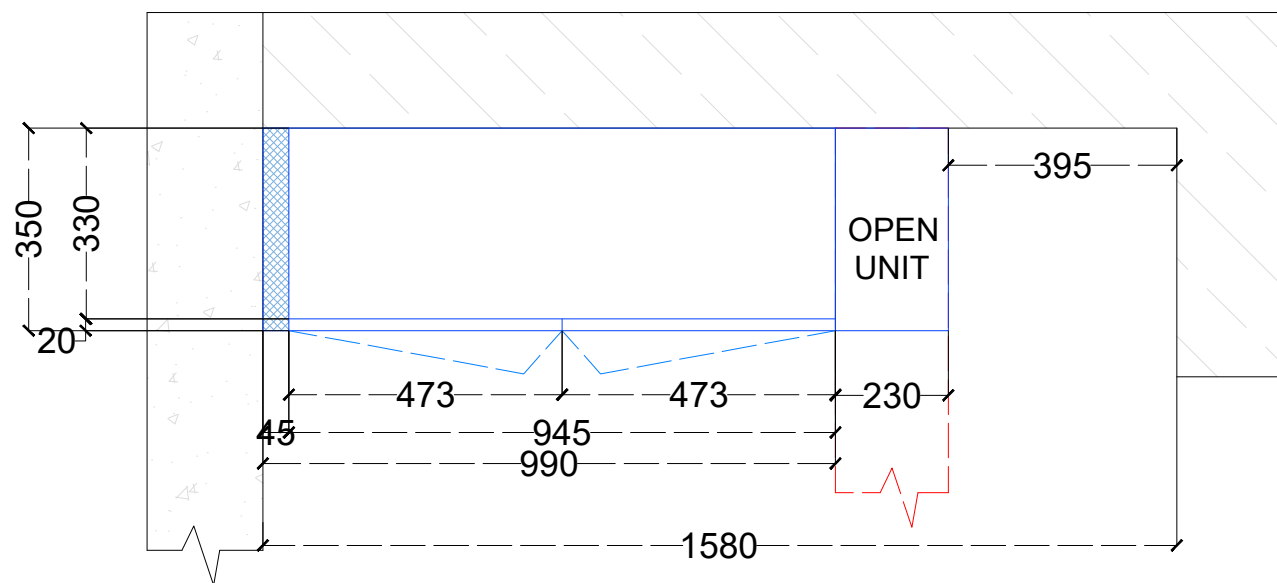
UTILITY - WALL UNIT PLAN
