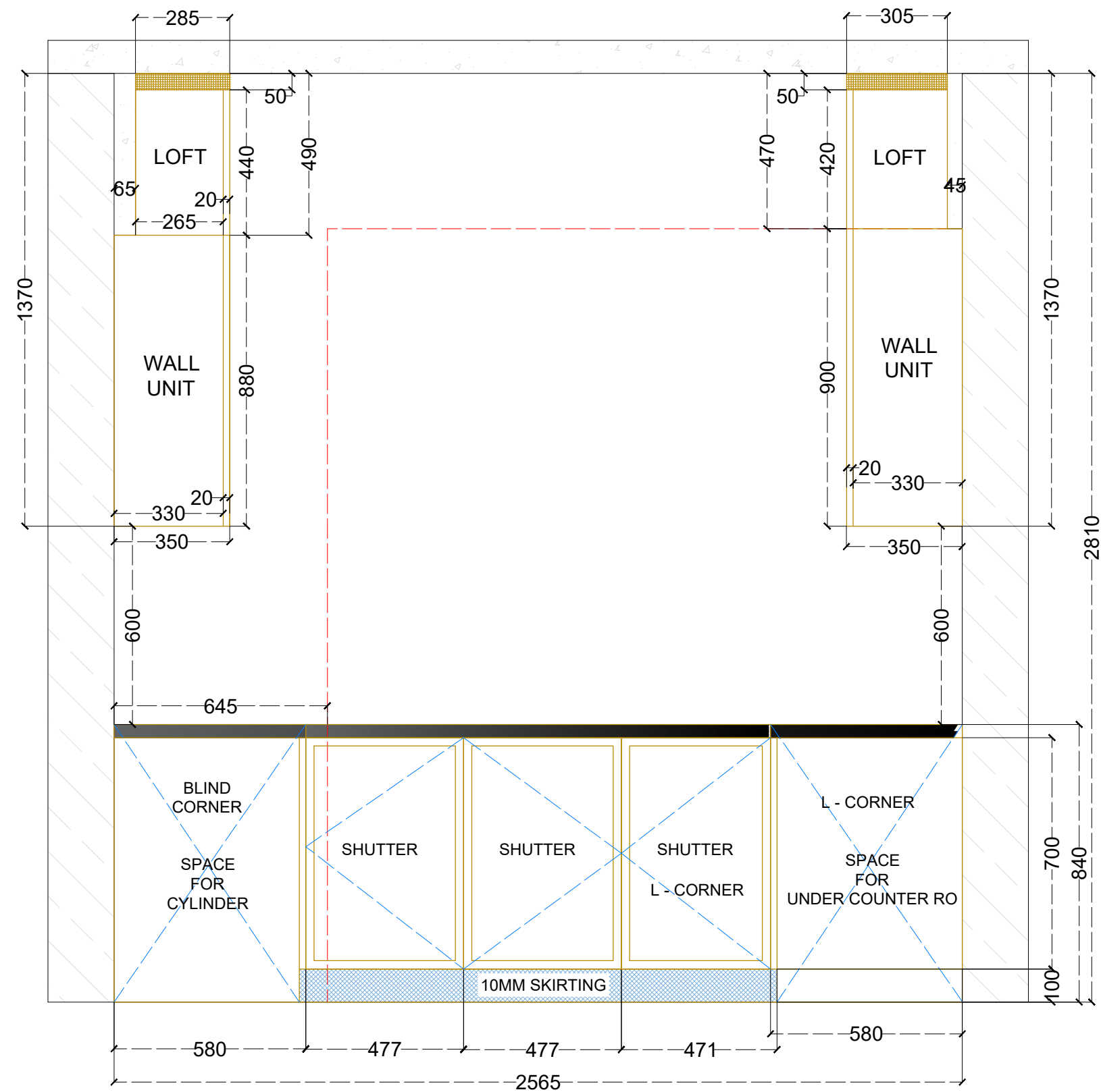
KITCHEN - ELEVATION B
