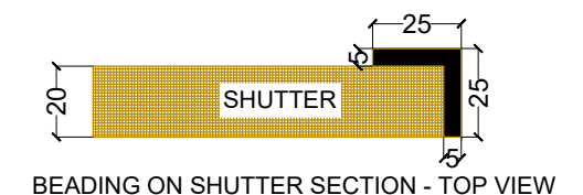
BEADING ON SHUTTER SECTION - TOP VIEW
