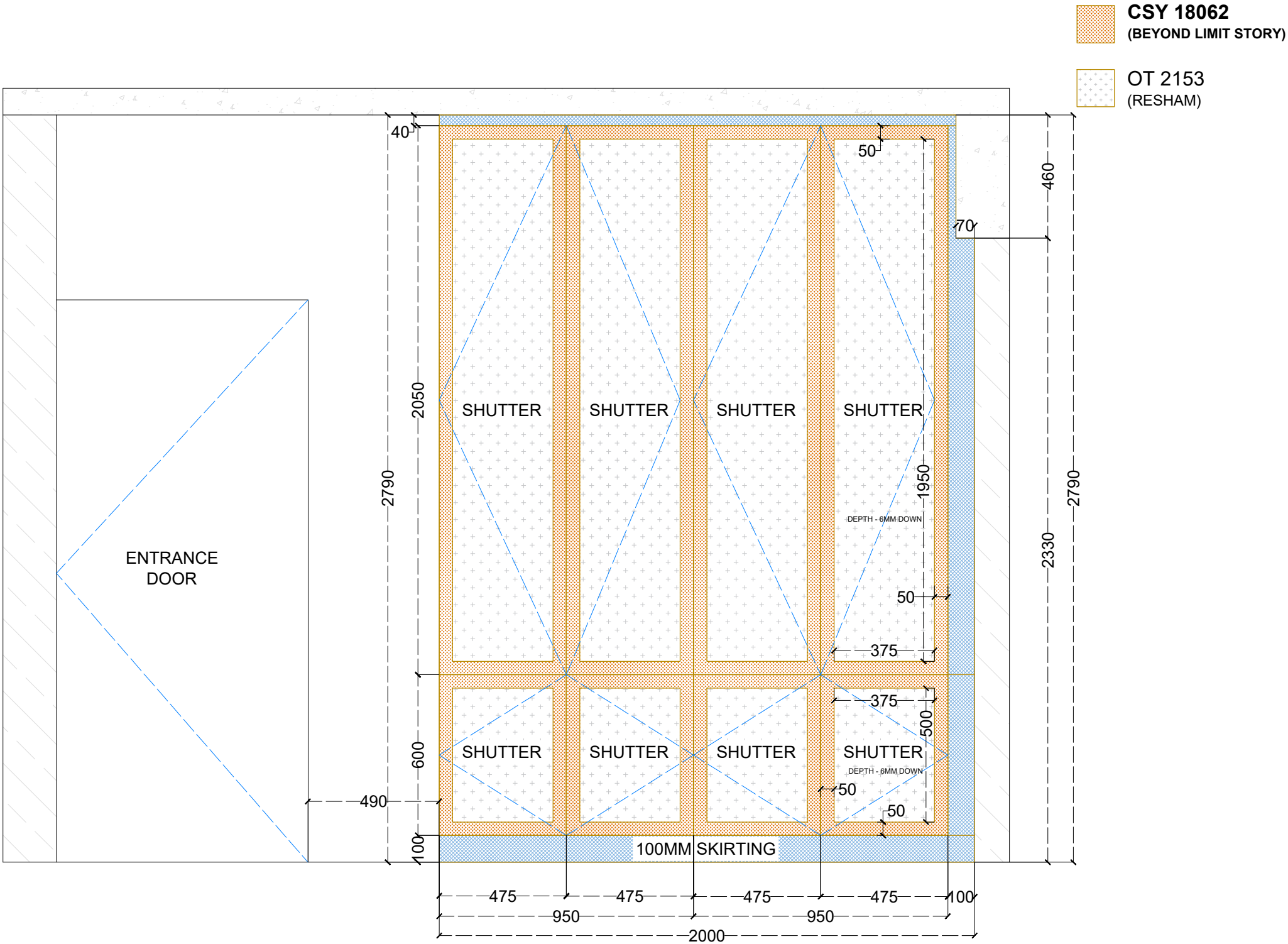
PBR WARDROBE - ELEVATION
