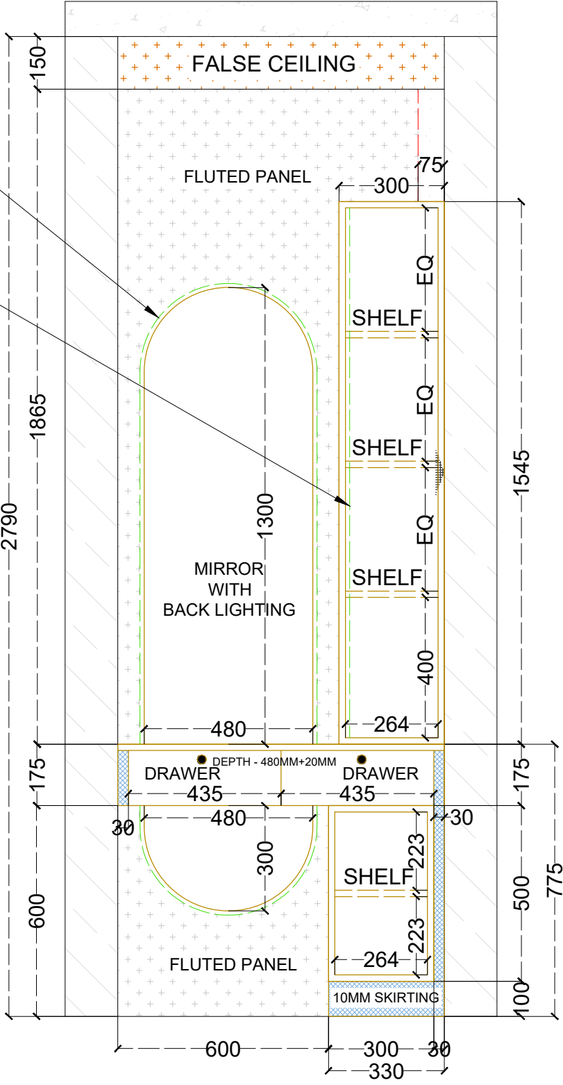
MBR DRESSER - INTERNAL
