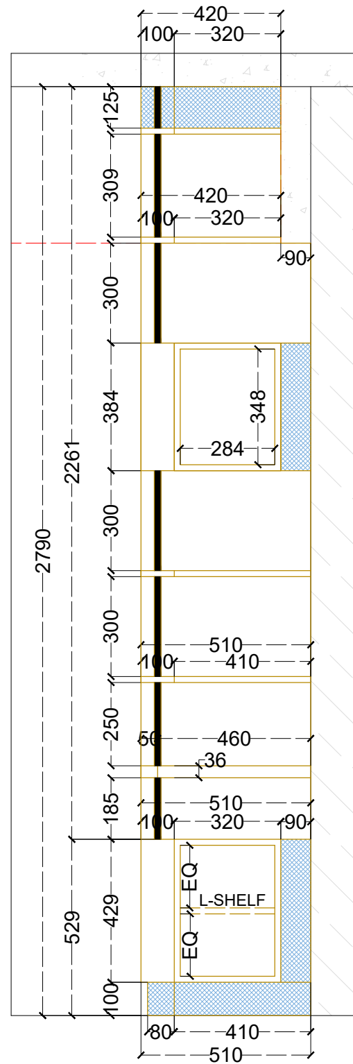
ELEVATION C - INTERNAL KBR WARDROBE - ELEVATION B INTERNAL (OPEN SHELVES & STORAGE)
