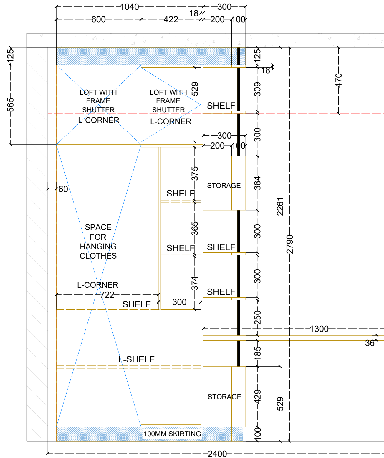
ELEVATION C - INTERNAL KBR WARDROBE - ELEVATION B INTERNAL (OPEN SHELVES & STORAGE)
