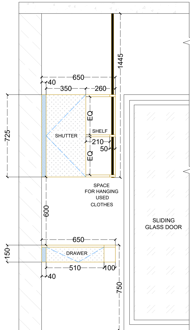
PBR STUDY - ELEVATION
