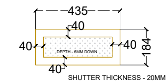
SHUTTER DETAIL (QTY - 4Nos)
