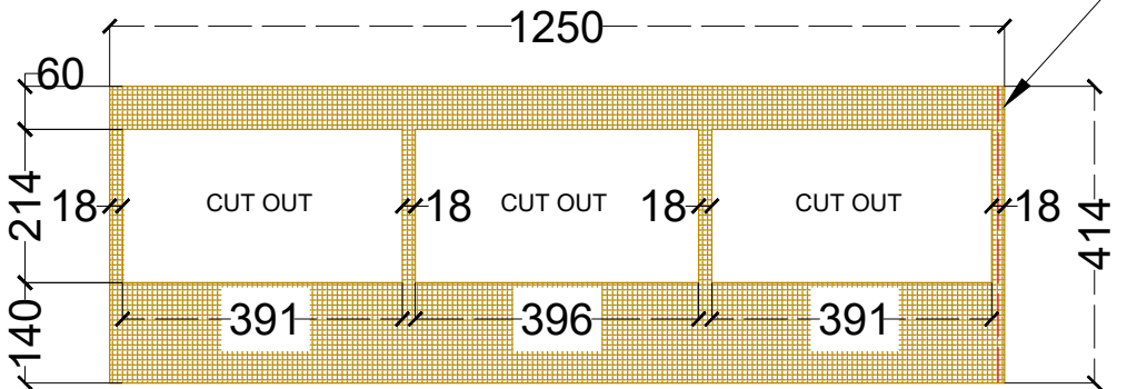
CARCASS FRONT PANEL DETAIL (18MM)
