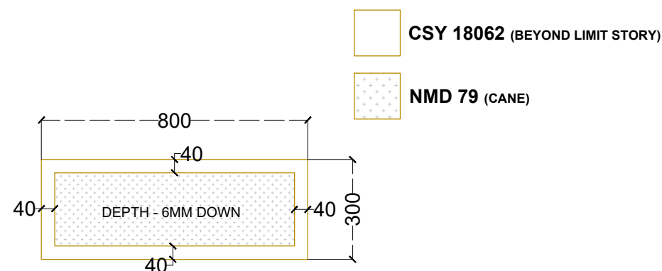
SHUTTER DETAIL (QTY 2Nos)
