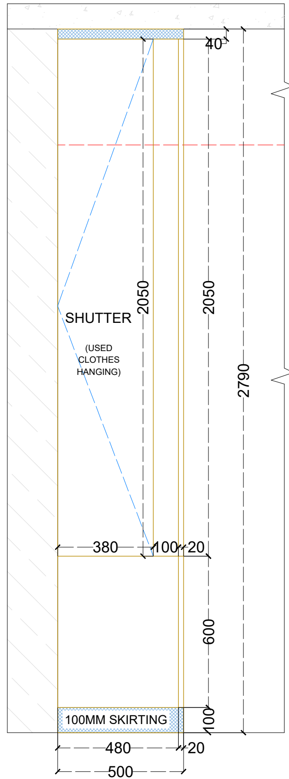
PBR WARDROBE - ELEVATION A-A
