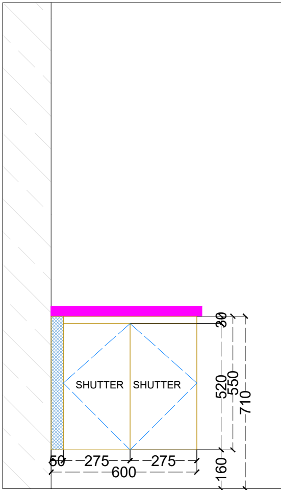
MBR VANITY - ELEVATION
