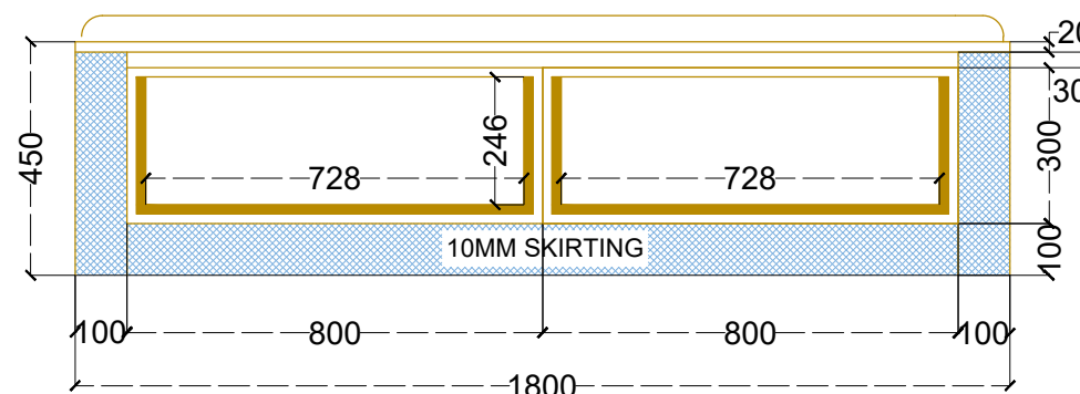
DINING - SEATER WITH STORAGE - INTERNAL
