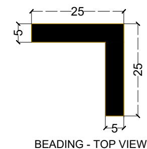
BEADING - TOP VIEW
