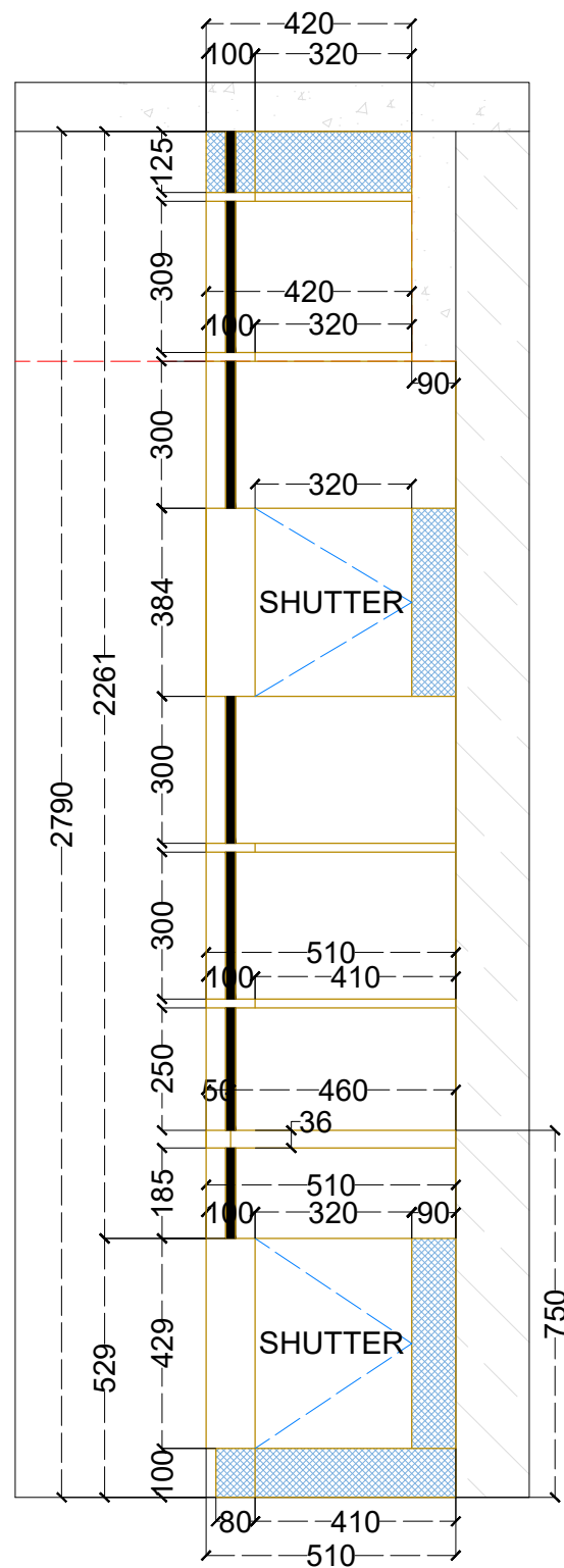
ELEVATION C (OPEN SHELF & STORAGE)
