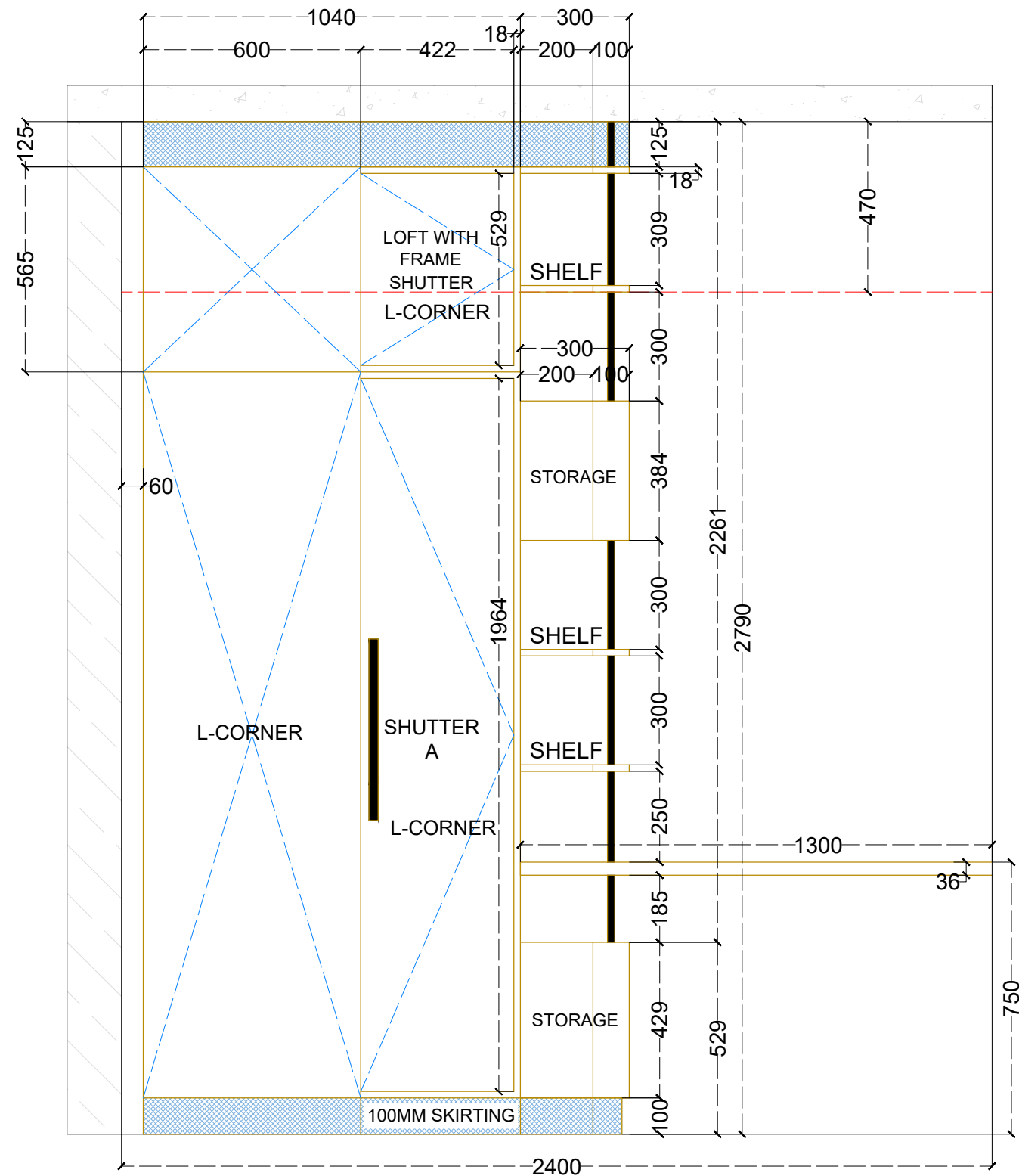
KBR WARDROBE - ELEVATION B
