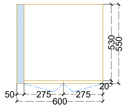
MBR VANITY - PLAN
