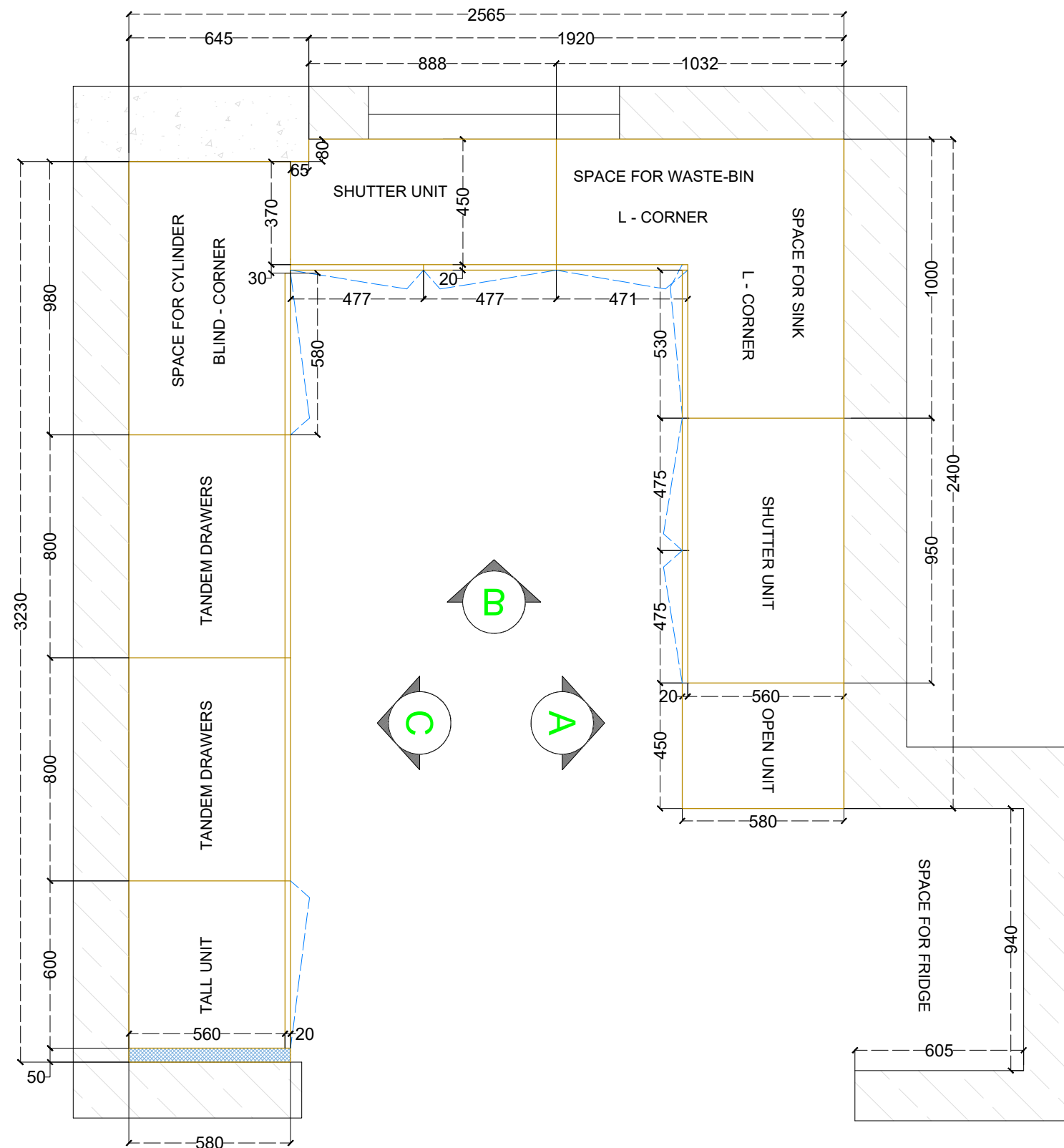
KITCHEN - BASE UNIT PLAN
