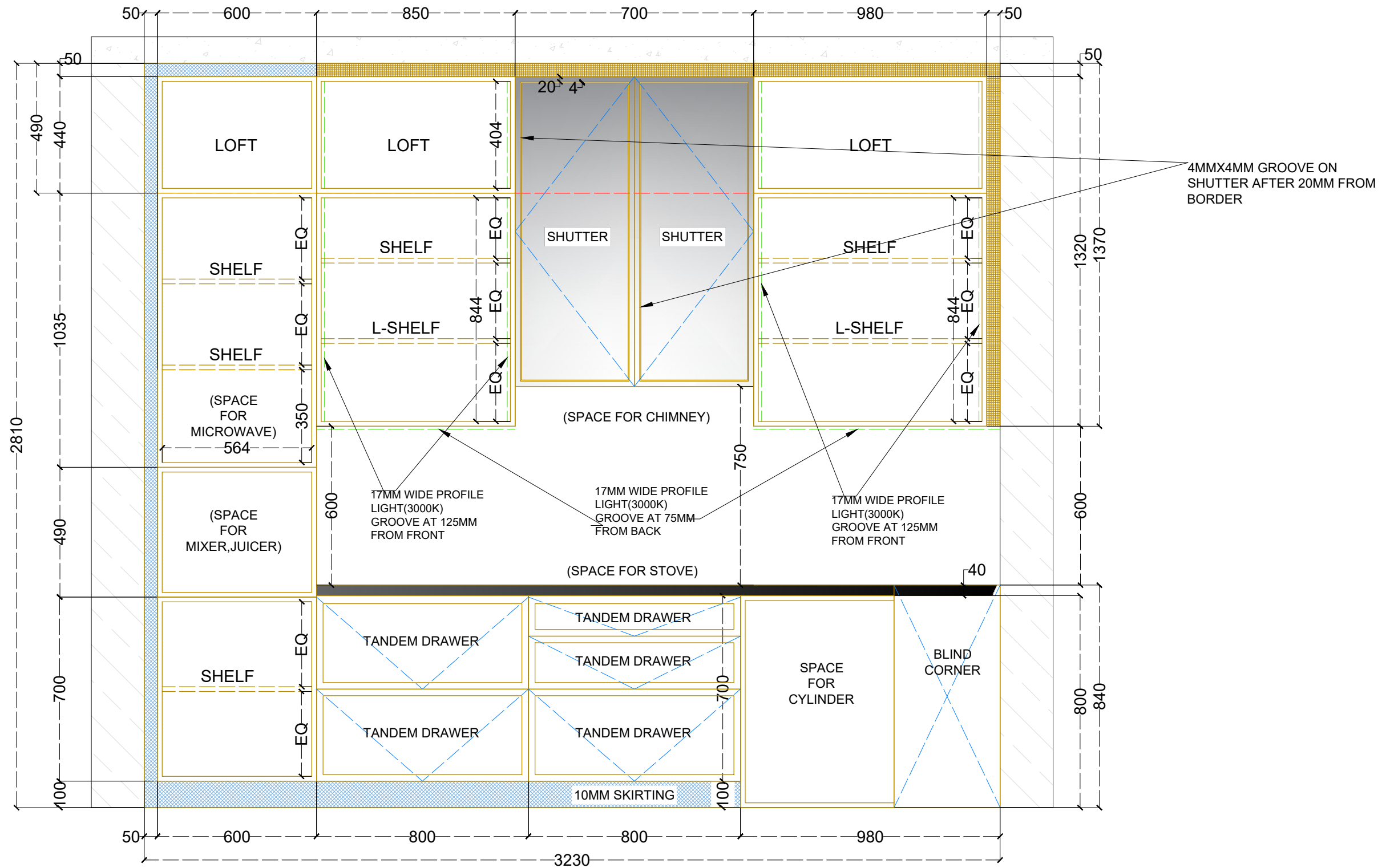
KITCHEN - ELEVATION C INTERNAL
