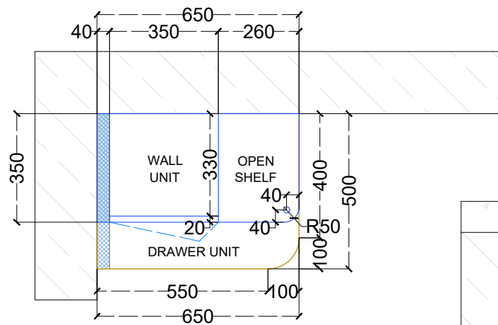
PBR STUDY - PLAN
