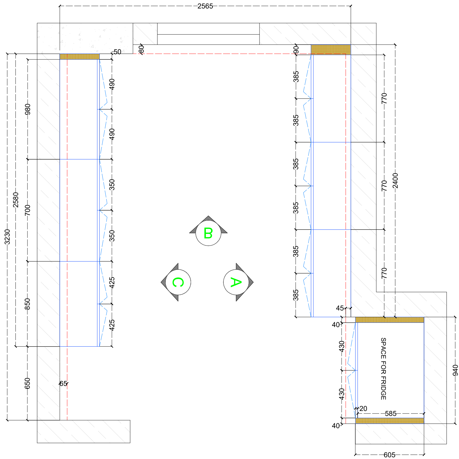
KITCHEN - WALL UNIT PLAN
