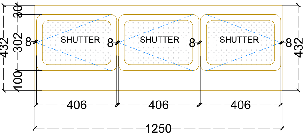
POOJA UNIT - ELEVATION
