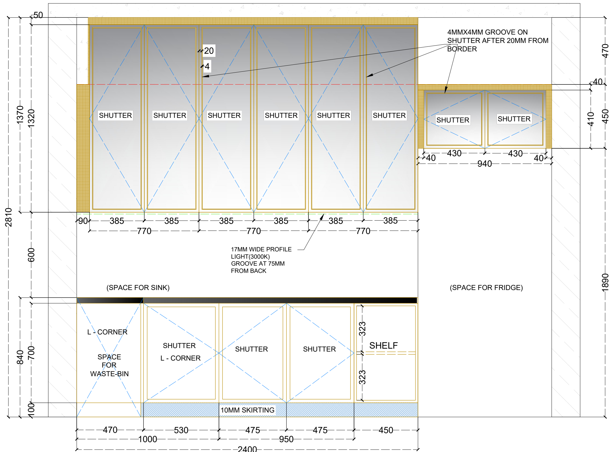
KITCHEN - ELEVATION A
