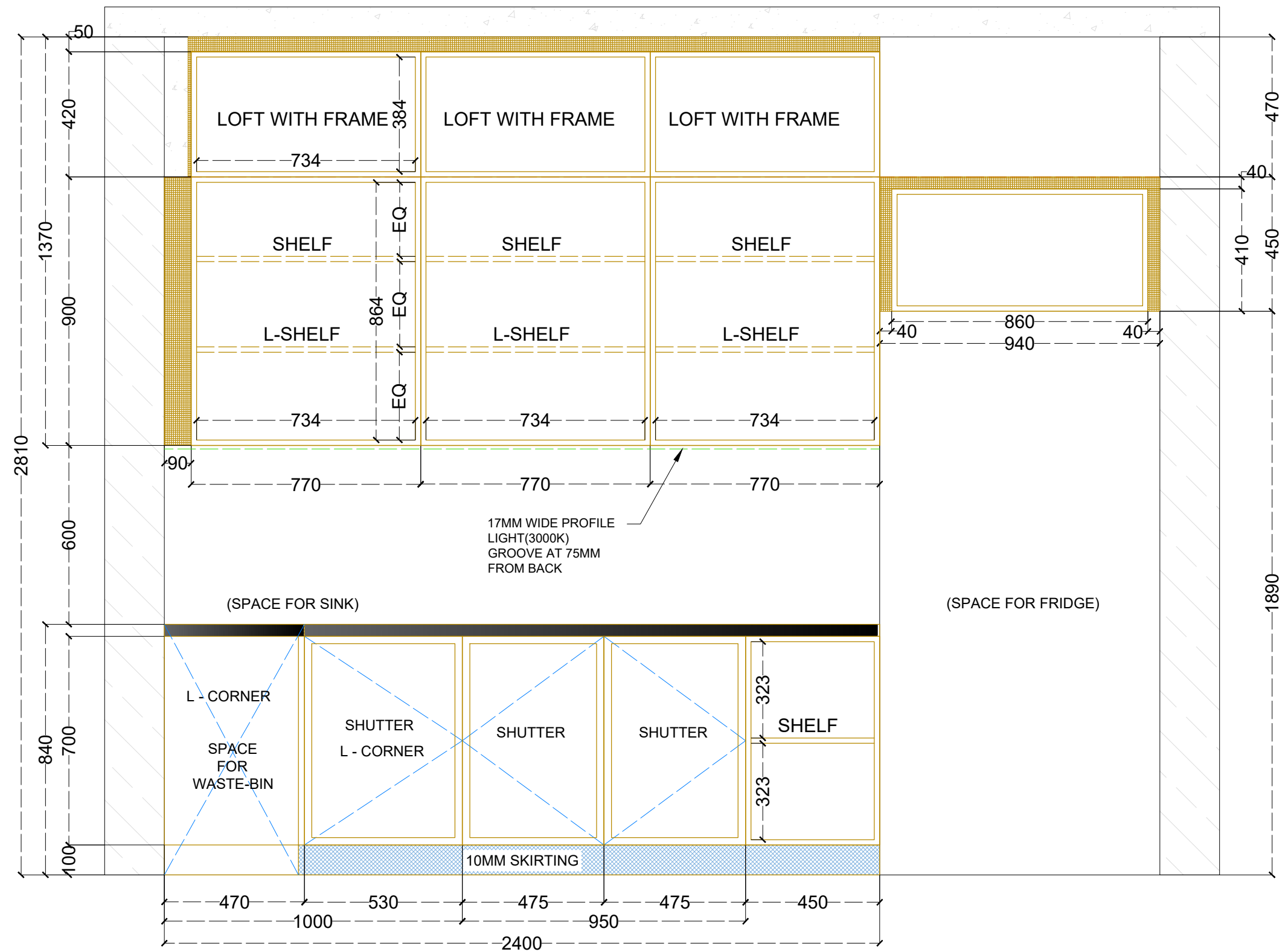
KITCHEN - ELEVATION A INTERNALS
