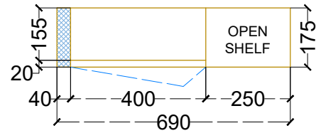
MBR VANITY - WALL UNIT PLAN
