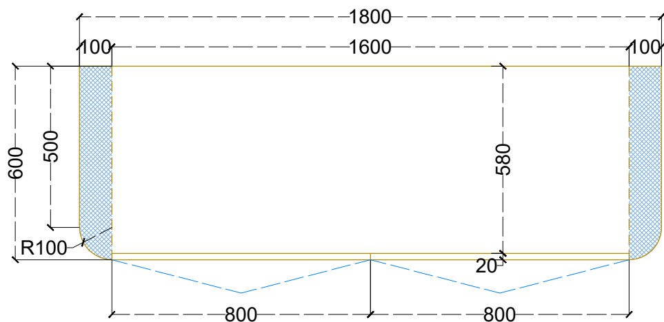
DINING - SEATER WITH STORAGE - PLAN
