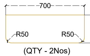
OPEN SHELF DETAIL
