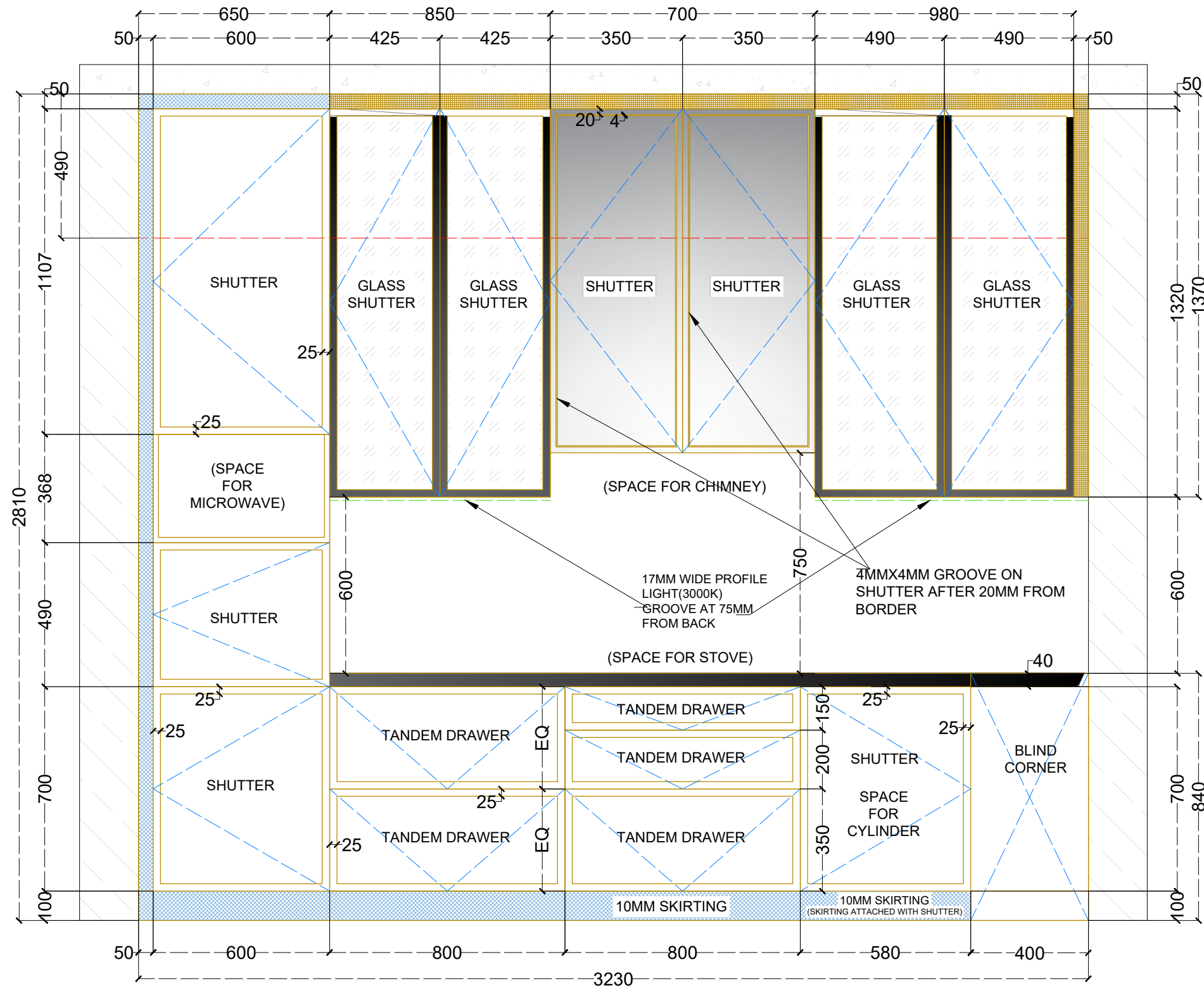
KITCHEN - ELEVATION C
