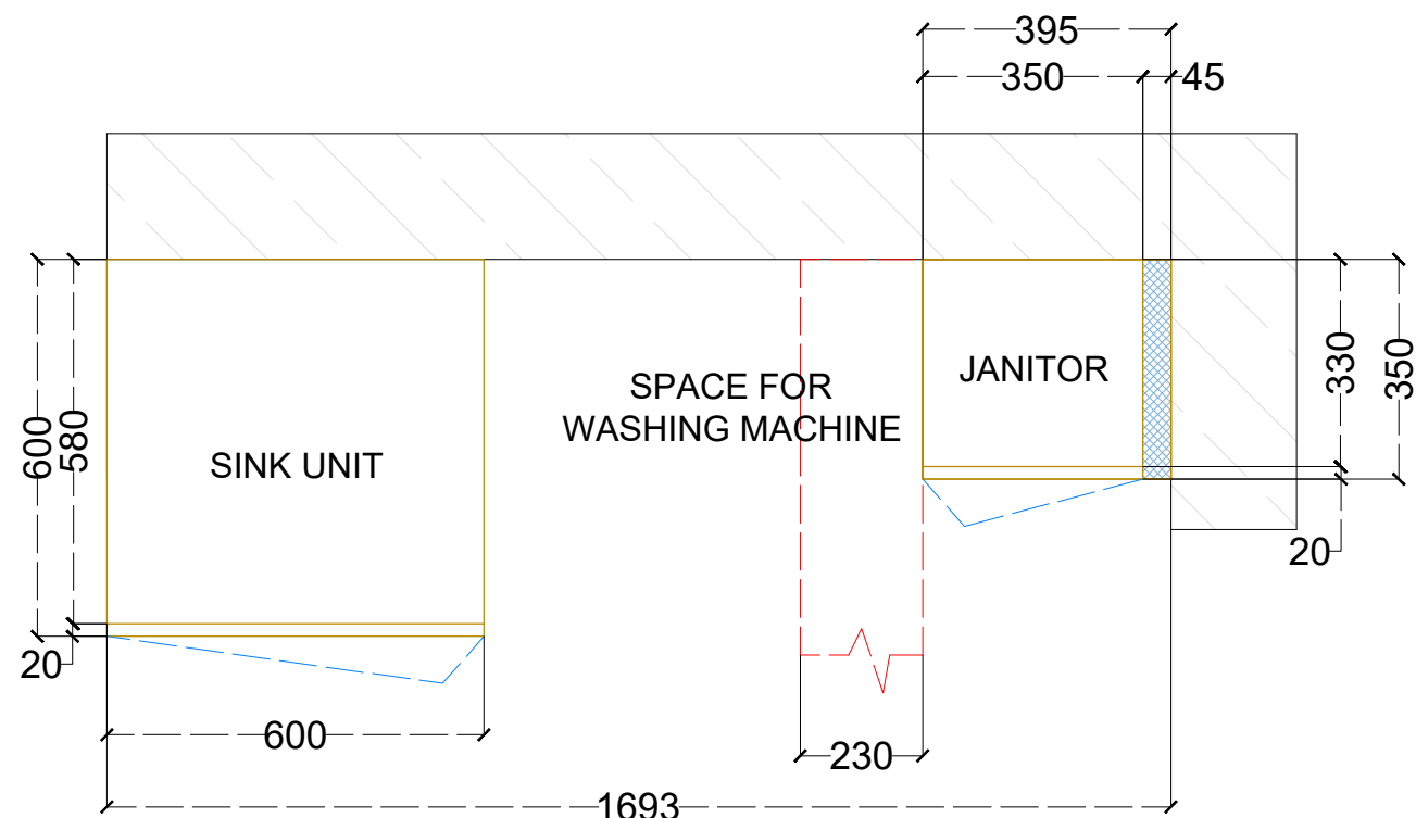
UTILITY - BASE UNIT PLAN
