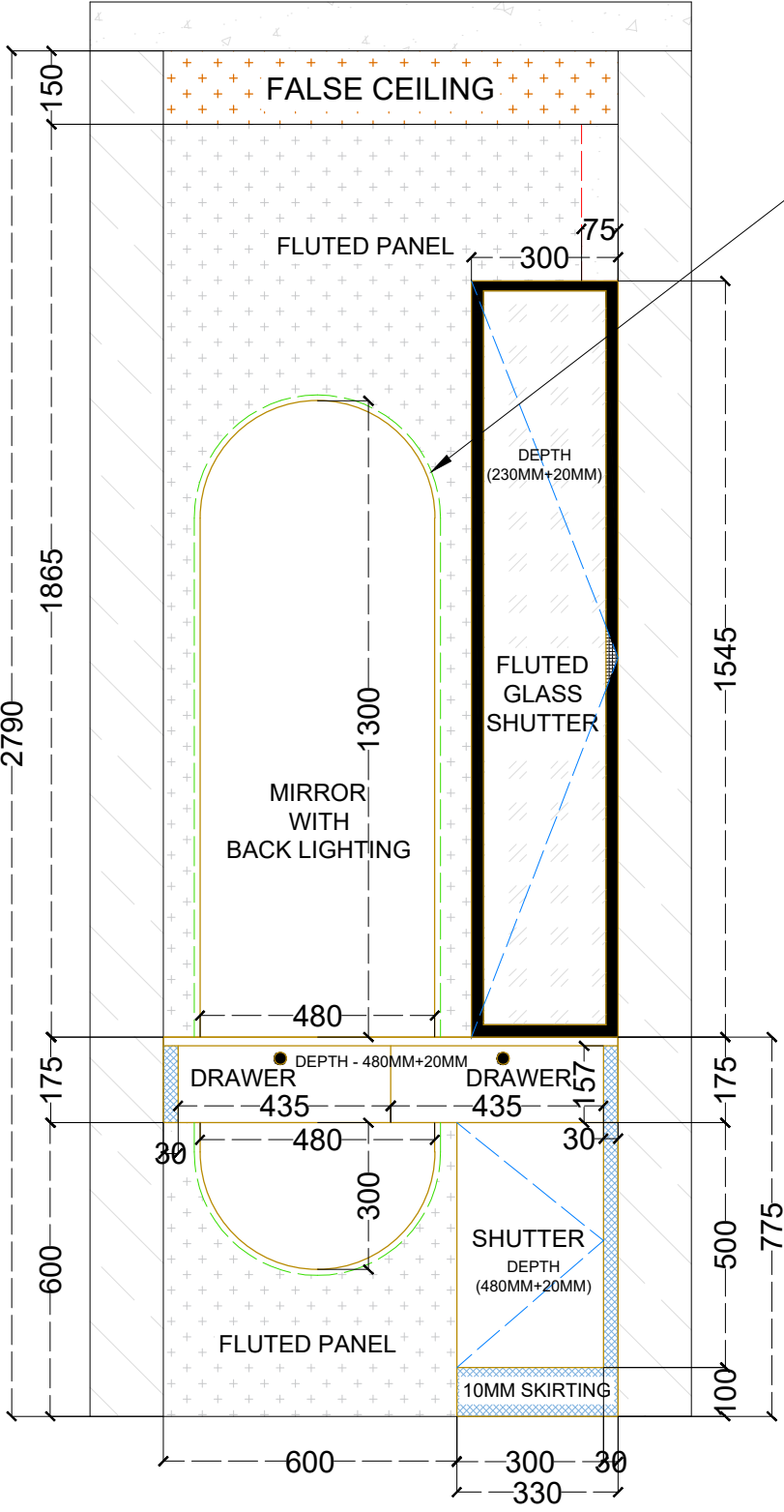
MBR DRESSER - ELEVATION
