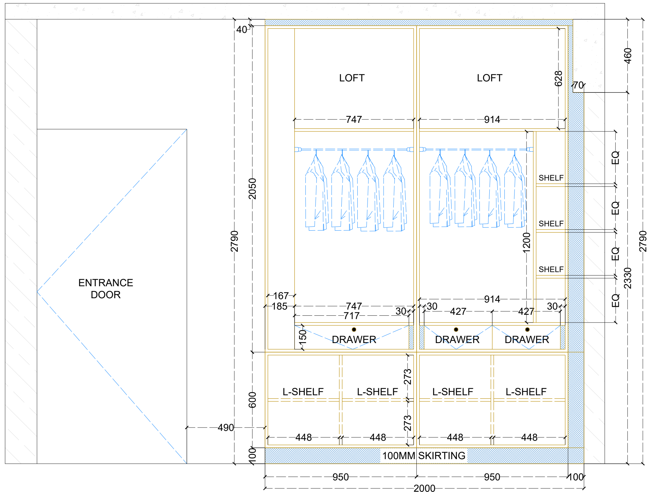
PBR WARDROBE - INTERNAL
