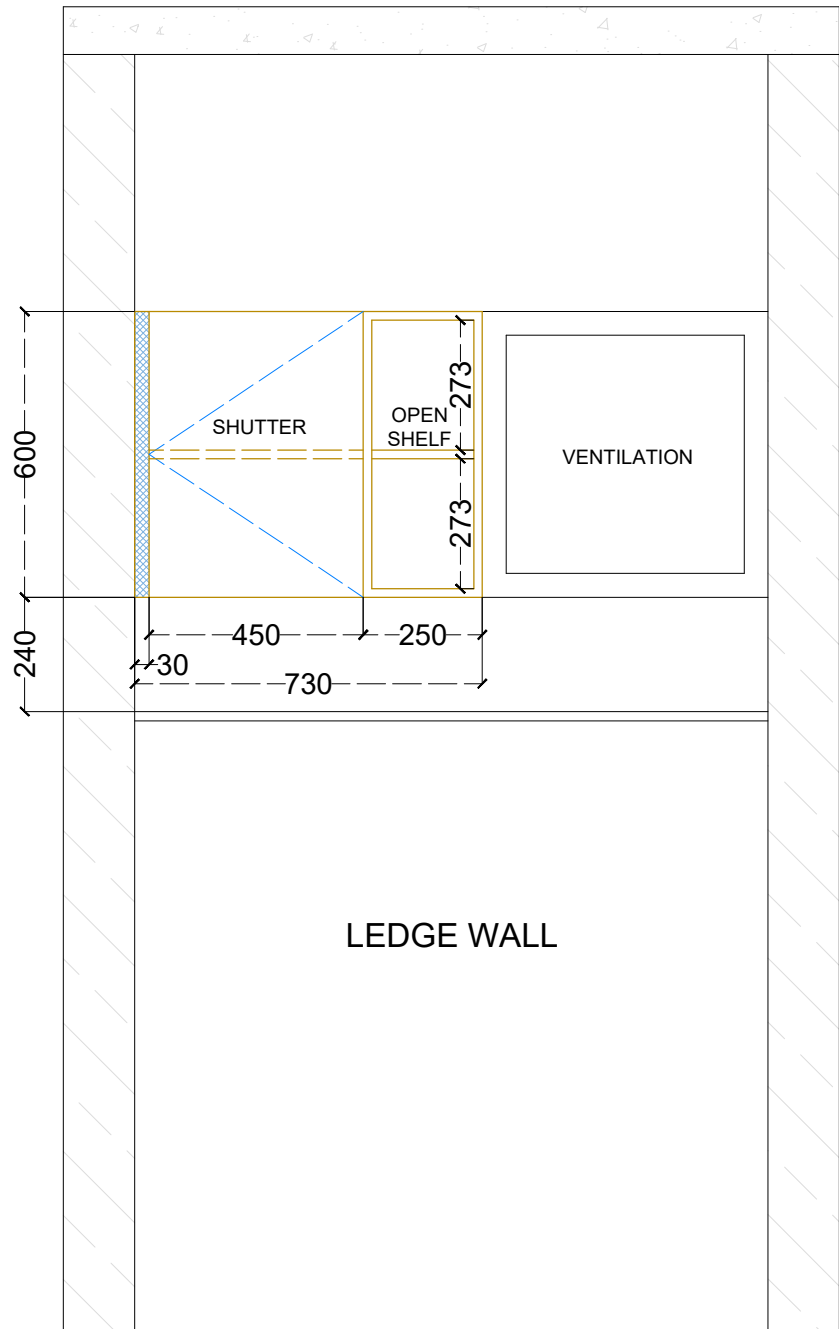
COMMON VANITY - WALL UNIT ELEVATION
