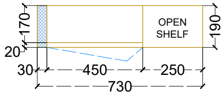
COMMON VANITY - WALL UNIT PLAN
