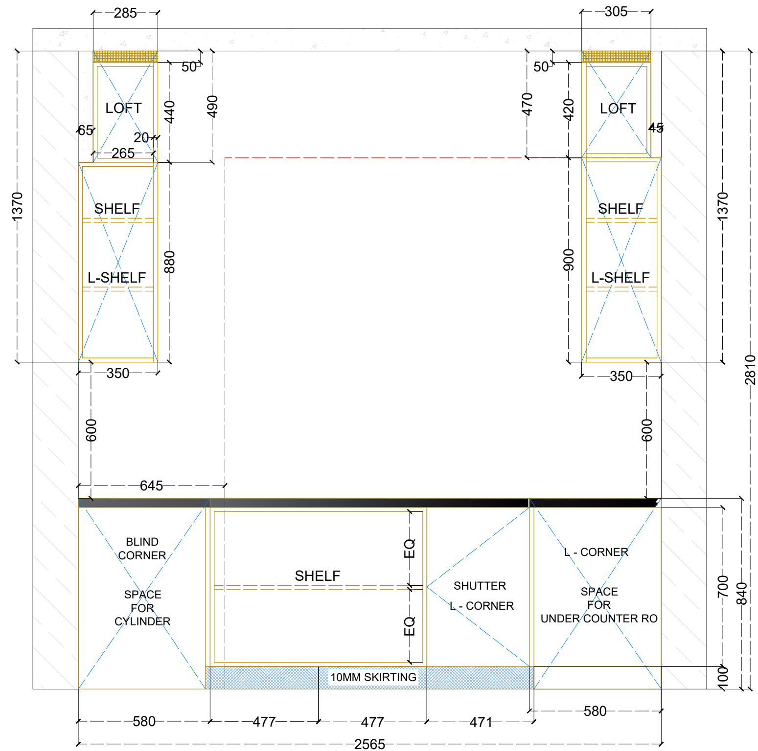
KITCHEN - ELEVATION B INTERNAL
