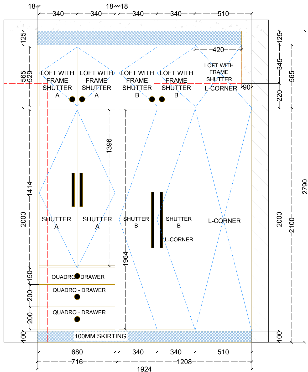
KBR WARDROBE - ELEVATION A
