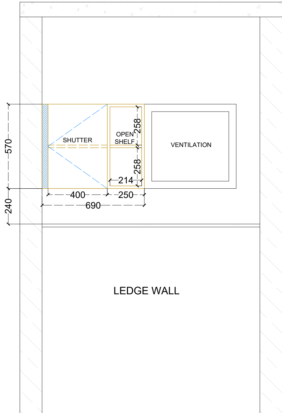
MBR VANITY - WALL UNIT ELEVATION
