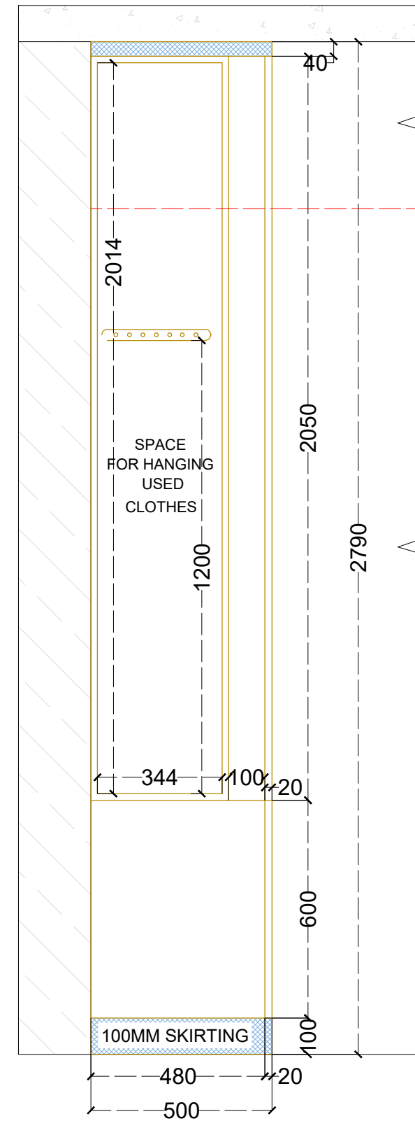
PBR WARDROBE - ELEVATION A-A INTERNAL
