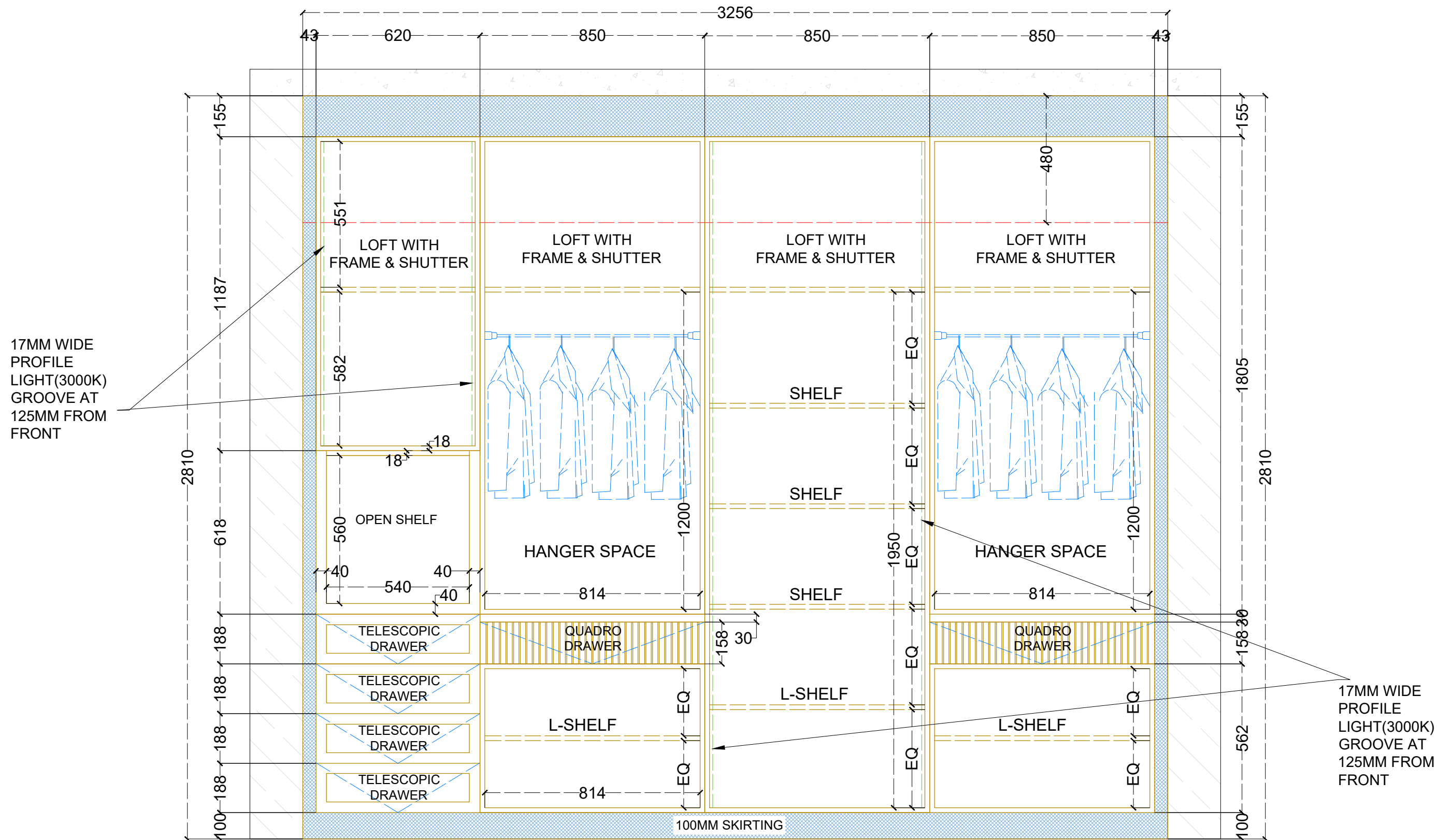
MBR WARDROBE - INTERNAL
