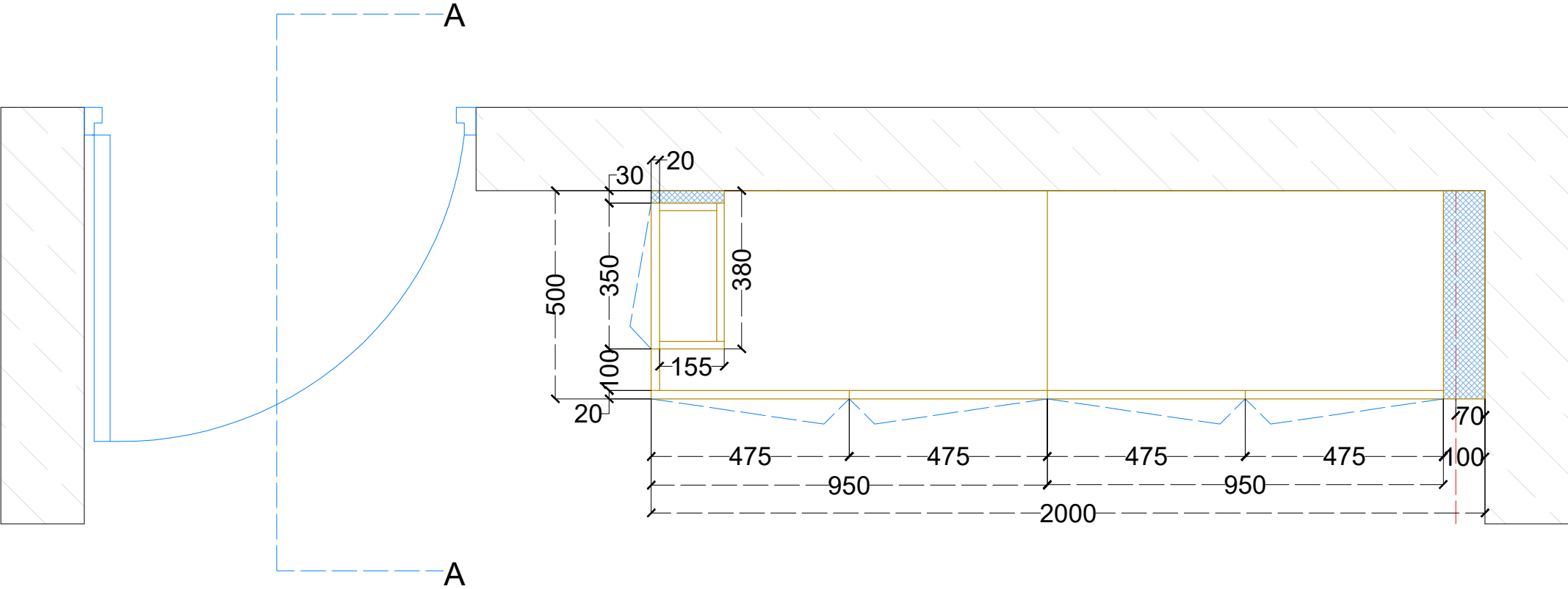
PBR WARDROBE - PLAN
